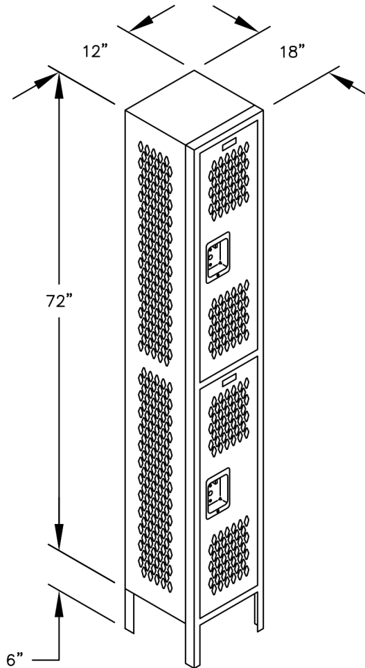
MODEL #72168 DOUBLE TIER VENTED LOCKER— 1 WIDE
